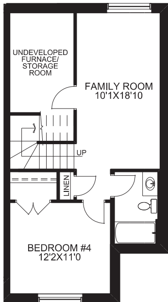
OPT'L BASEMENT DEV. 457 SQ.FT. DEVELOPED
