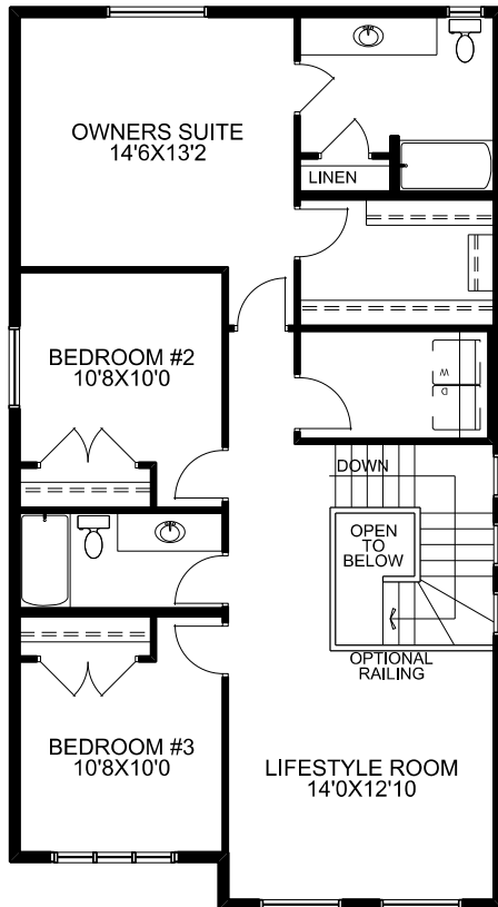
UPPER FLOOR PLAN #1 3 BEDROOM - PROPEL ENSUITE
