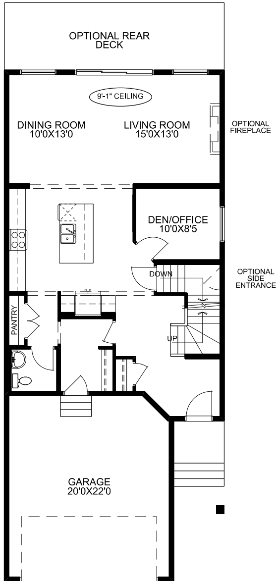
MAIN FLOOR PLAN #1 DEN - HALF BATH - PANTRY
