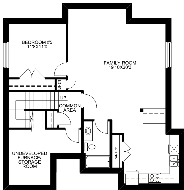
OPT'L BASEMENT SUITE 885 SQ.FT. DEVELOPED
