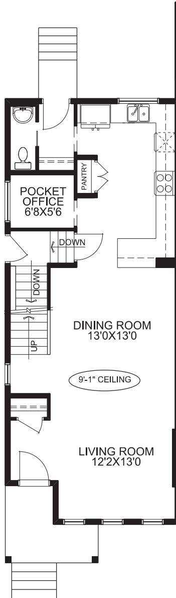
MAIN FLOOR PLAN
