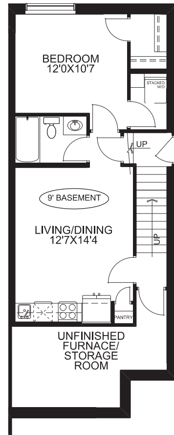
OPT'L BASEMENT DEV 508 SQ.FT. DEVELOPED
