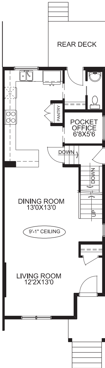
MAIN FLOOR PLAN
