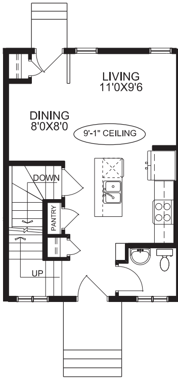
MAIN FLOOR PLAN
