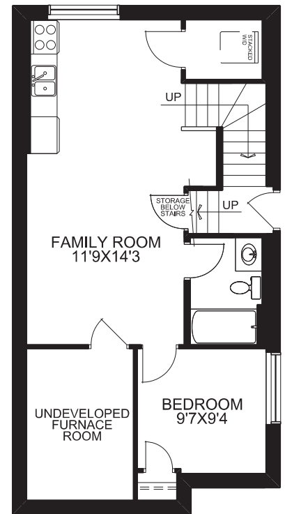
OPT'L BASEMENT DEV. 509 SQ.FT. DEVELOPED
