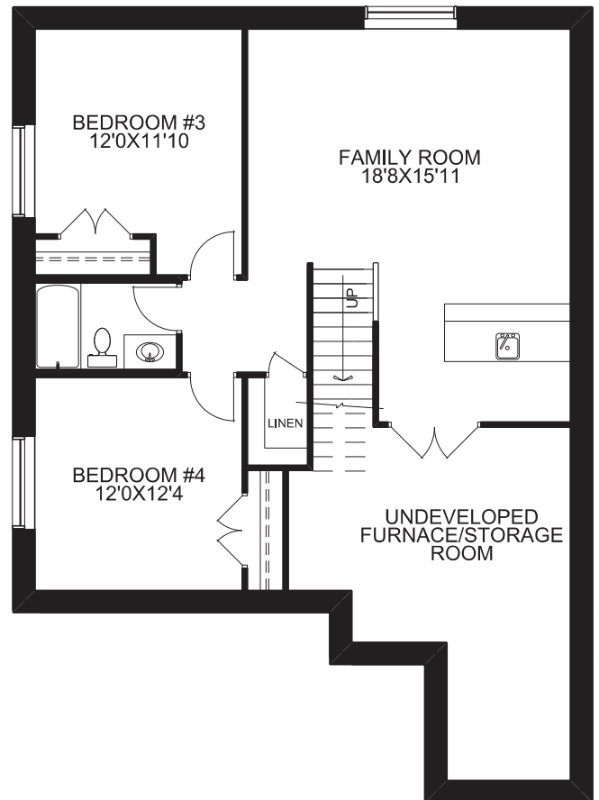
OPT'L BASEMENT DEVELOPMENT 873 SQ.FT. DEVELOPED
