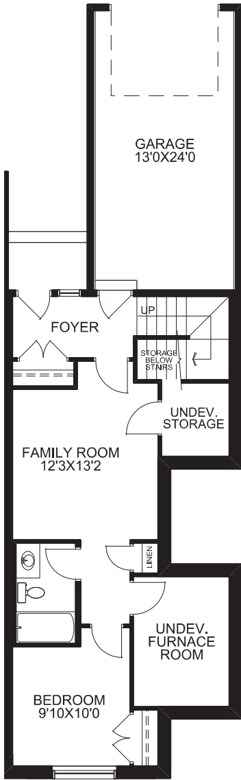
BASEMENT DEVELOPMENT
