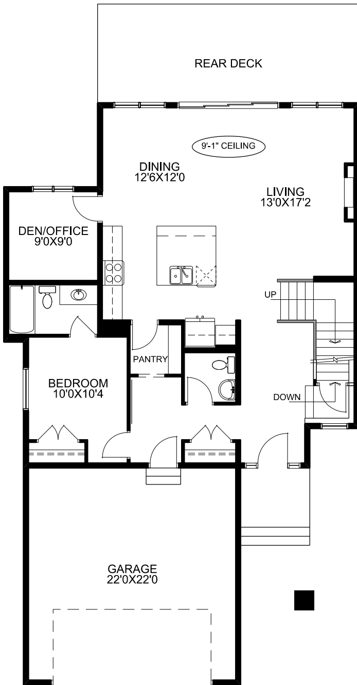
OPTIONAL MAIN FLOOR PLAN W/ BEDROOM & FULL BATH 1206 SQ.FT.
