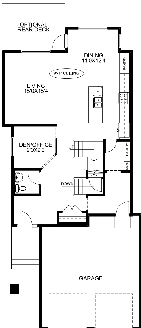
Main Floor
