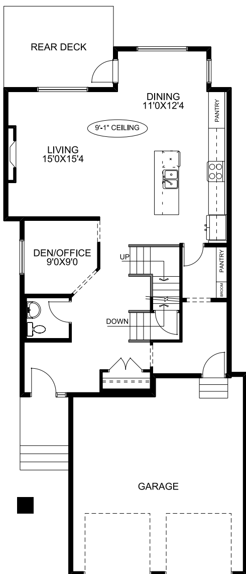
Main Floor
