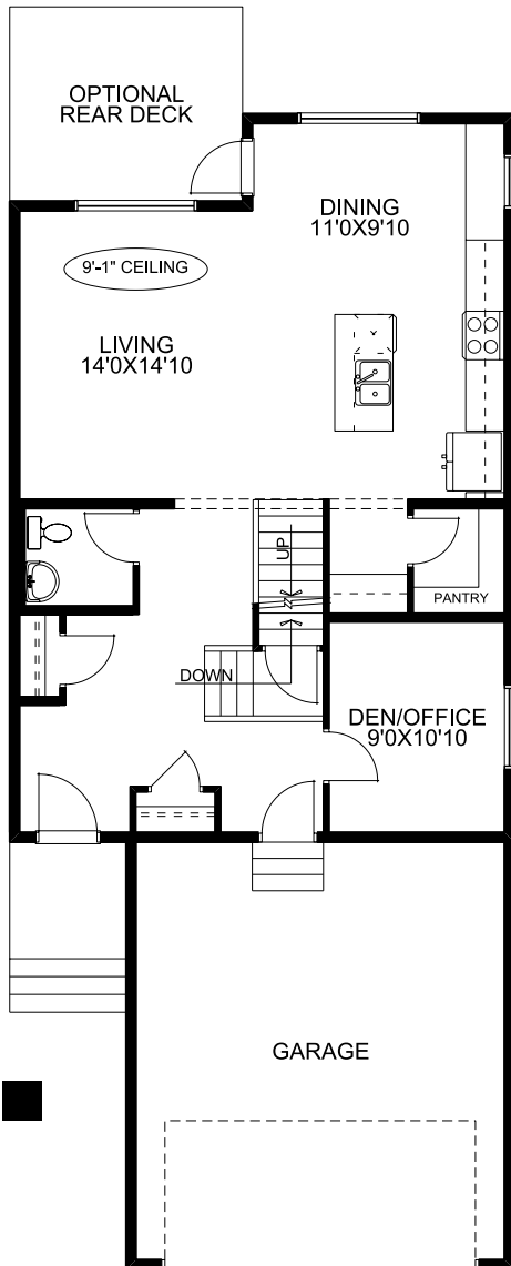
Main Floor
